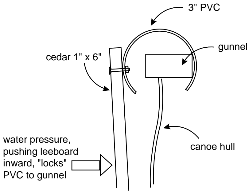
LEEBOARD DETAIL (looking aft)
