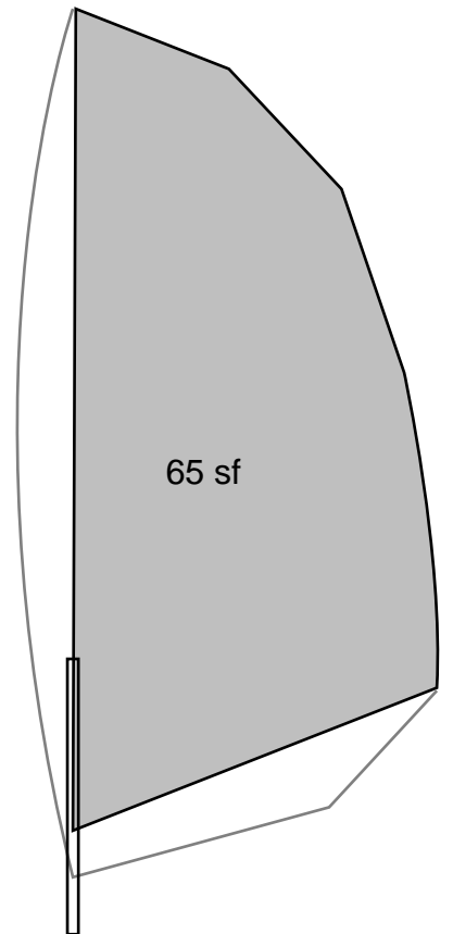
4. WINDSURFER GUNTER (AR 3.5:1)
